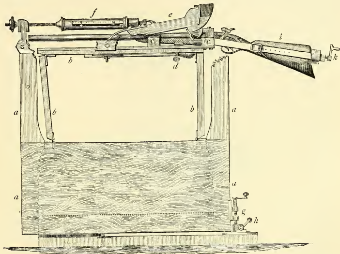
“The Field” Machine Gun Rest.
